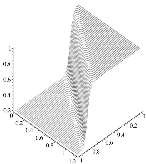
Fig. 16. Shock propagation, \lambda = 0.01 .
