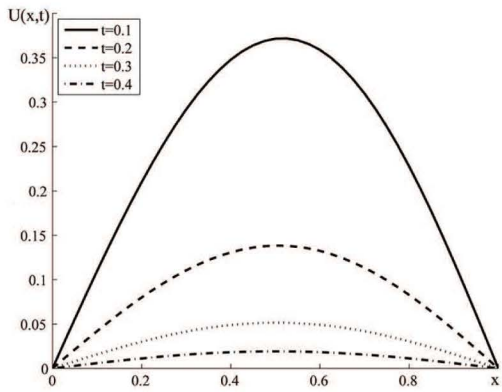
Fig. 2. Solutions for \lambda=1 , N=40 , \Delta t=0.0001 .
