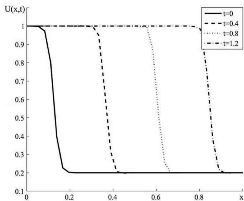
Fig. 13. Solutions for \lambda = 0.005 .
