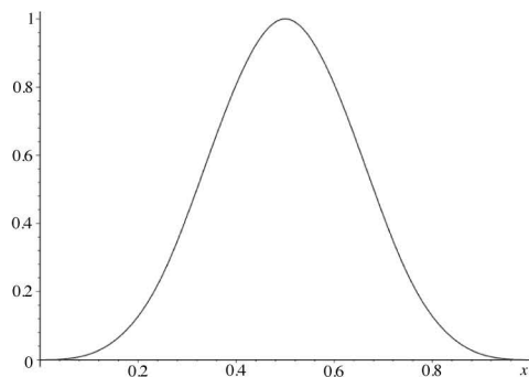
Fig. 1. Exponential cubic B-splines over the interval [0, 1].
