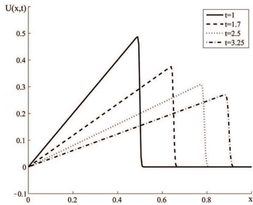
Fig. 11. Shock propagation, \lambda = 0.0005 .
