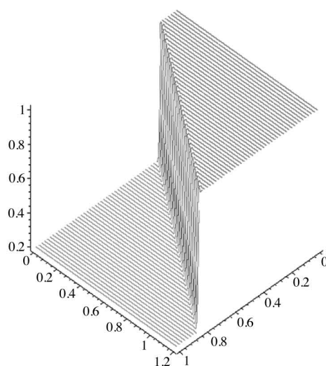
Fig. 17. Shock propagation, \lambda = 0.005 .
