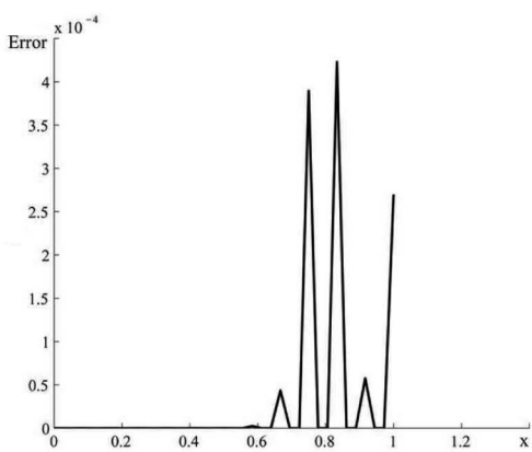
Fig. 14. L_2 error norm for \lambda = 0.01 , t = 1.2 .
