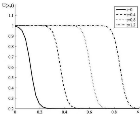
Fig. 12. Solutions for \lambda = 0.01 .
