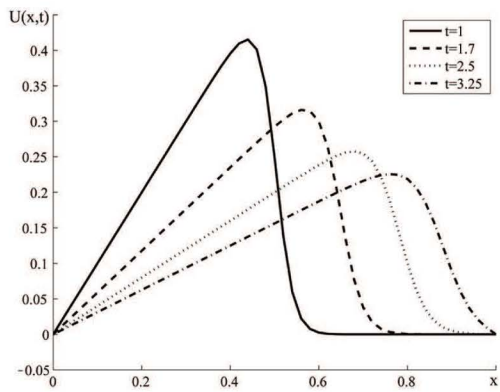
Fig. 10. Shock propagation, \lambda = 0.005 .
