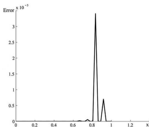
Fig. 15. L_2 error norm for \lambda = 0.005 , t = 1.2 .
