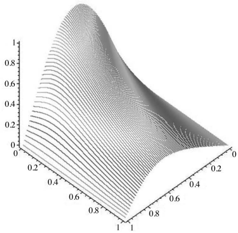
Fig. 7. Solutions for \lambda = 0.1 , N = 40 , \Delta t = 0.01 .
