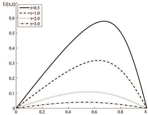
Fig. 3. Solutions for \lambda=0.1 , N=40 , \Delta t=0.0001 .
