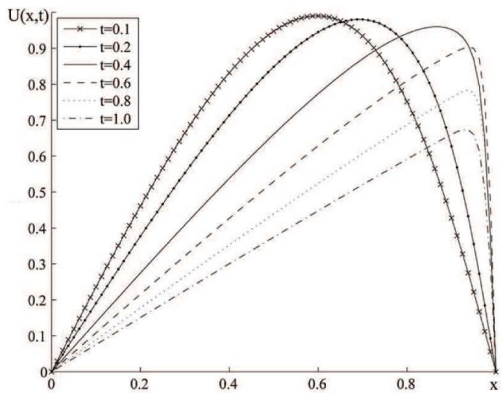
Fig. 4. Solutions for \lambda=0.01 , N=80 , \Delta t=0.0001 .
