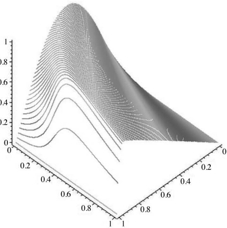
Fig. 8. Solutions for \lambda = 0.01 , N = 80 , \Delta t = 0.01 .
