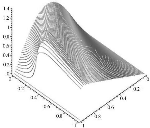
Fig. 9. Solutions for \lambda = 0.001 , N = 80 , \Delta t = 0.001 .
