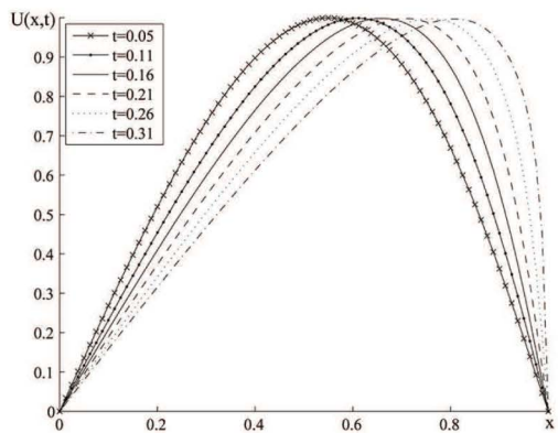
Fig. 5. Solutions for \lambda=0.001 , N=80 , \Delta t=0.0001 .
