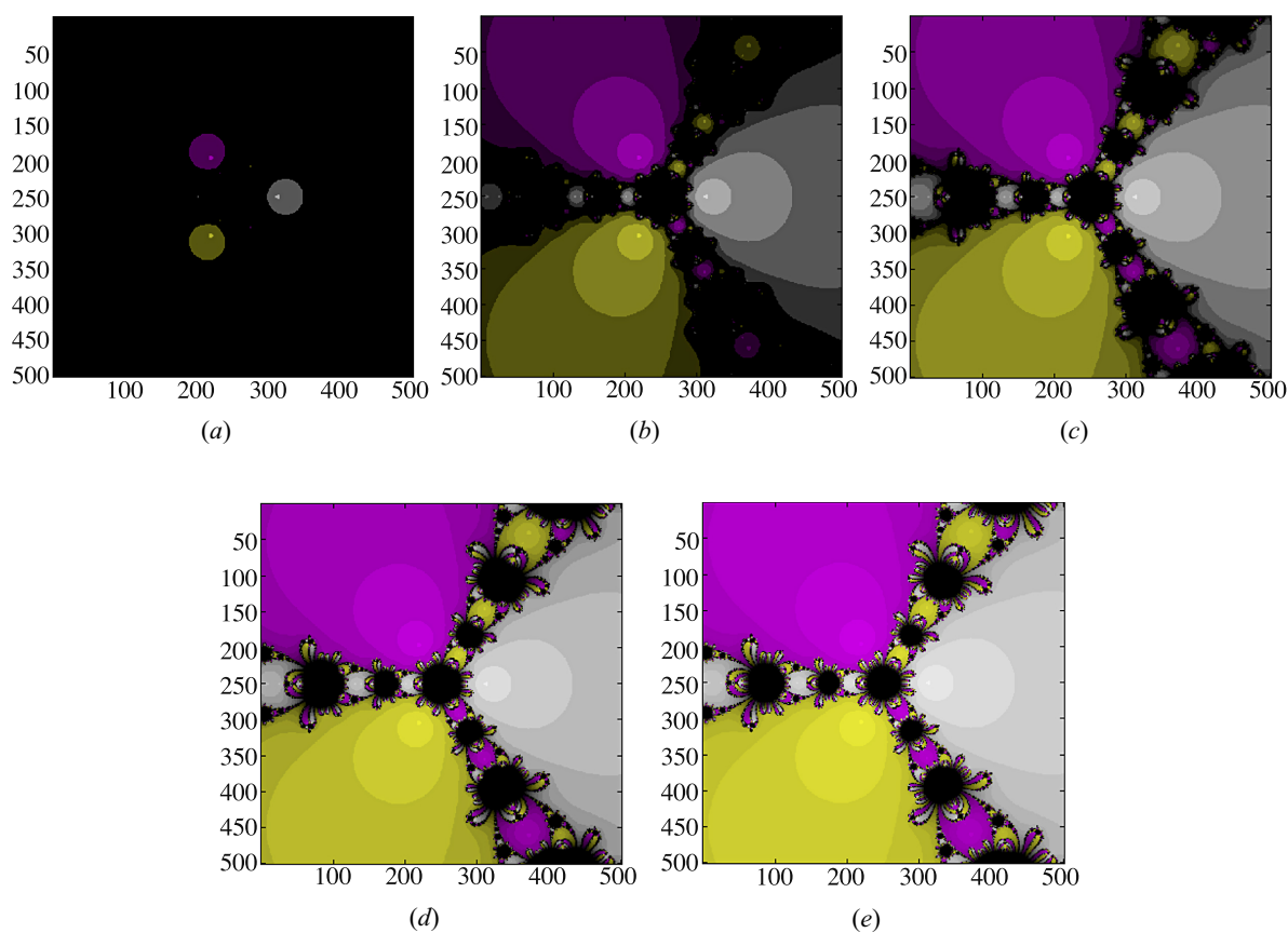
Fig. 3. Dynamics of the proposed method with 03 (a), 06 (b), 09 (c), 15 (d), and 21 (e) iterations for f_2 = z^3 - 1 .
