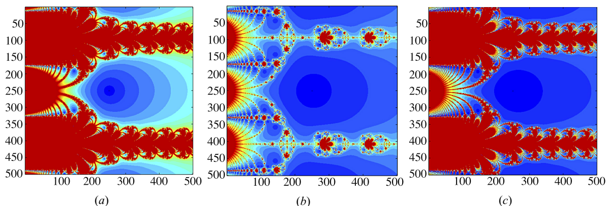
Fig. 1. Basin of attraction for e^x - 1 by Newton method (a), Jarratt method (b) and proposed method (c).
